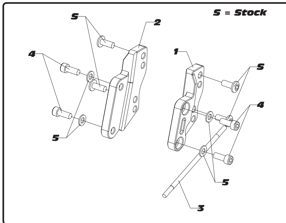
Parts Diagram
