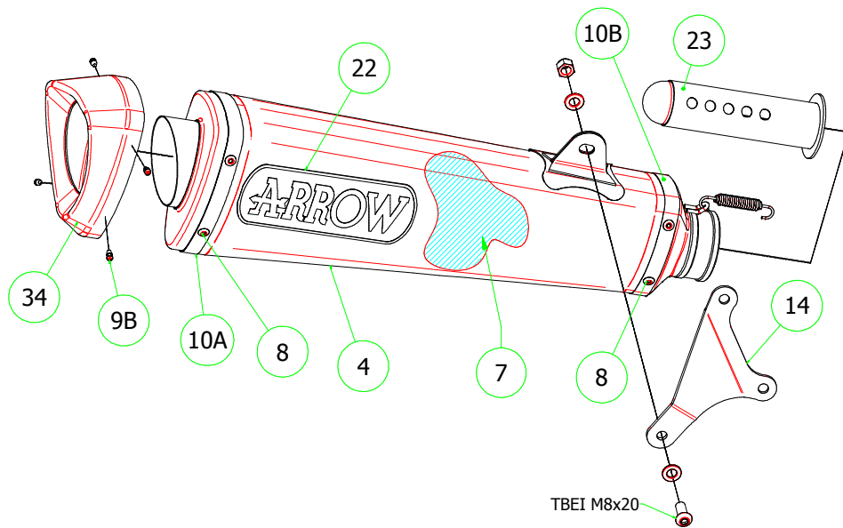
71197PRK Titanium-Carbon Silencer
