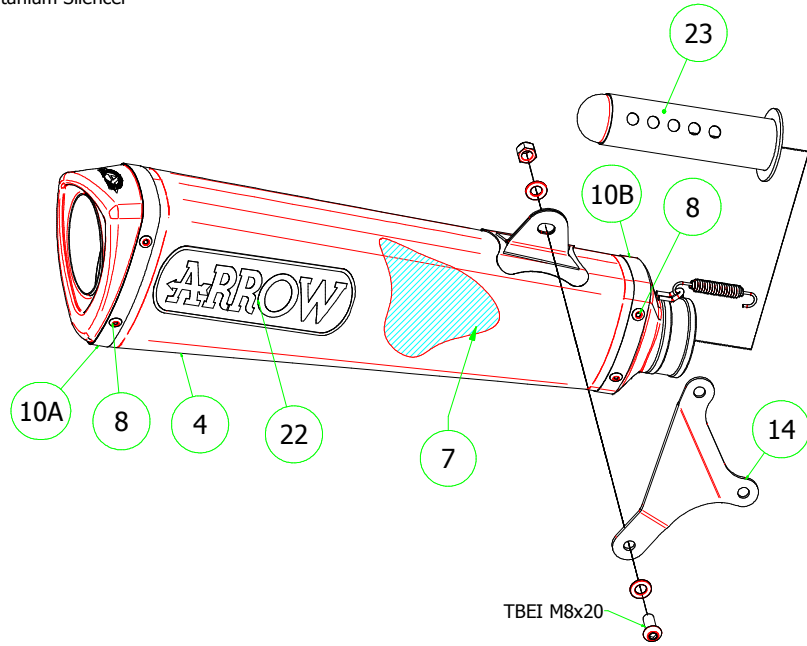
71197PR Titanium Silencer
